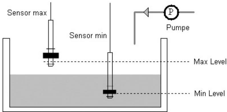
Fig. 3: aquaniveau with two float switches
